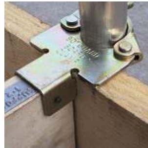
90° Board Clamp
